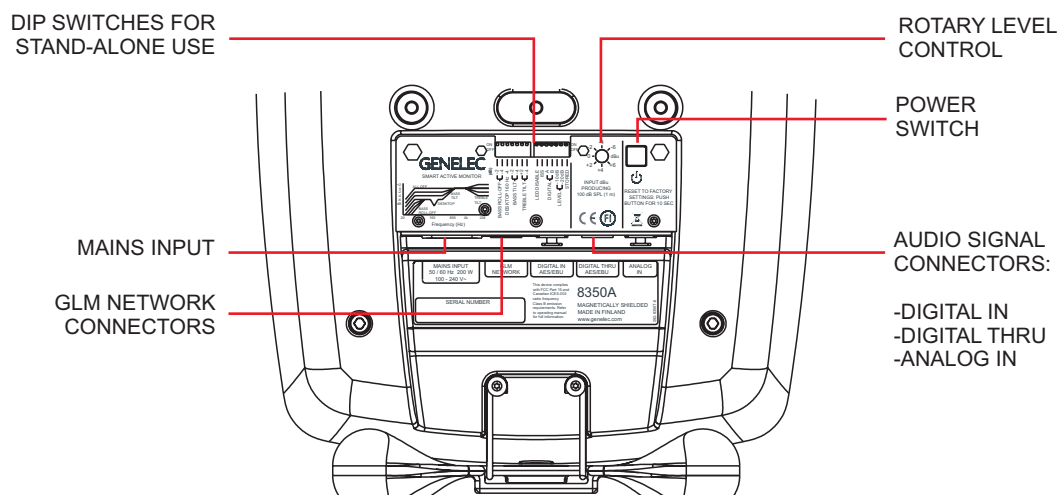
Figure 2. Connectors and controls on the back panel of a 8350A. 8340A shares the same layout.
