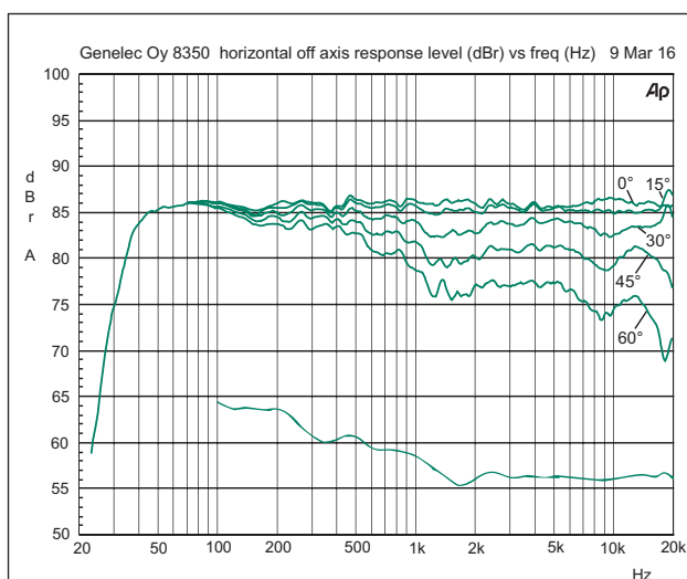
Figure 14. The upper curve group shows the horizontal directivity characteristics of the 8350A measured at 1 m. The lower curve shows the system's power response.
