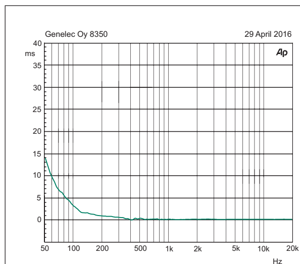
Figure 15. The curve above shows the delay variation of the 8350A as a function of frequency.
