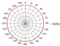
Polar Pattern of i825
