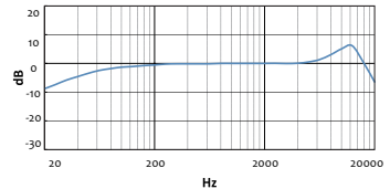
Typical Frequency Response of i825 at 50cm from the source
