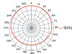
Polar Pattern of i855
