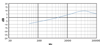
Typical Frequency Response of i855 at 50cm from the source
