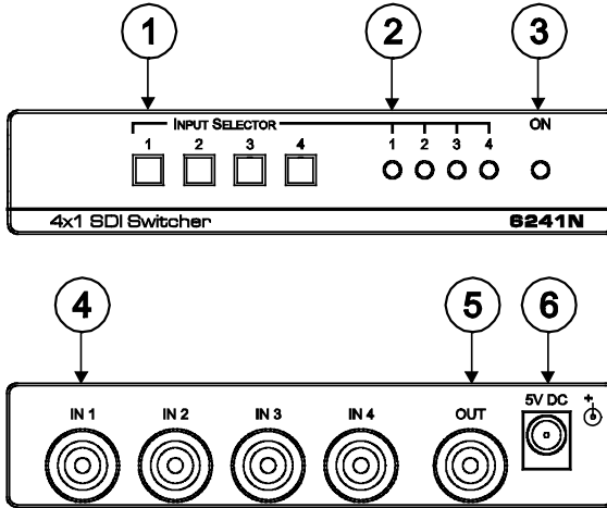
Figure 1: 6241N 4x1 SDI Switcher Functions
