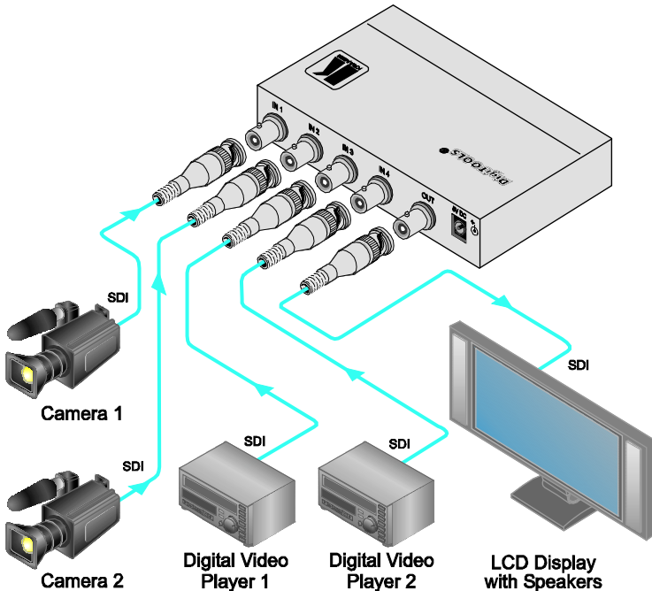
Figure 2: Connecting the 6241N 4x1 SDI Switcher
