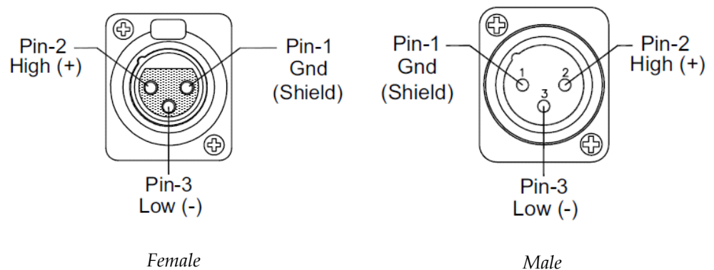
Figure 1–6 XLR Pin-Outs
