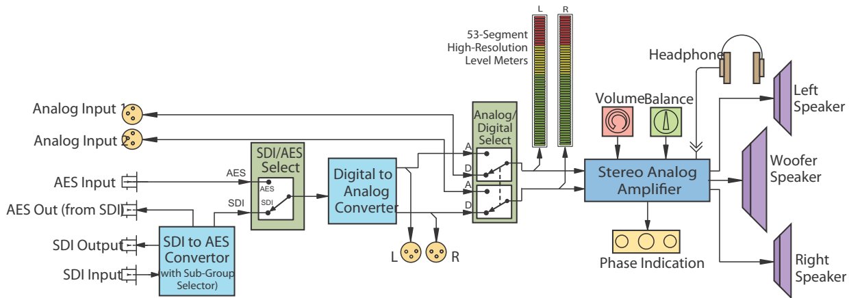
Figure 1–10 AMPx-SDA Block Diagram
