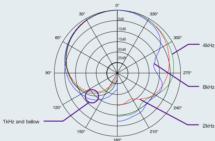
DRM85-C POLAR DIAGRAM
